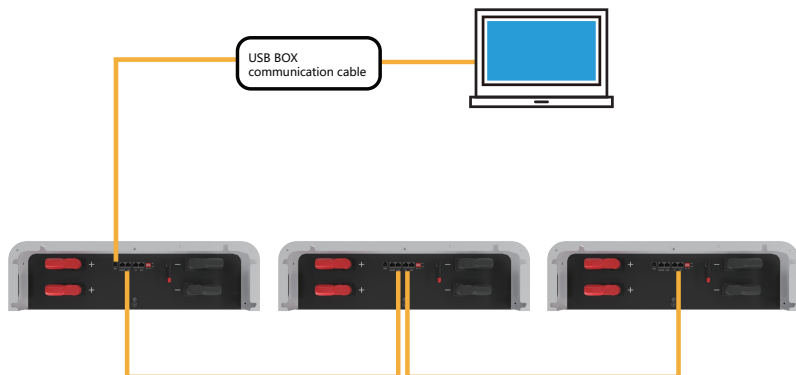
Figure 5-3: Communication Cable Connections between Battery and Computer
